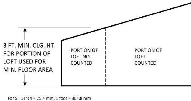
Figure AQ104.1.3 Loft Ceiling Height
